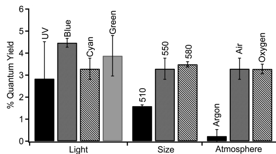
Figure 3. (Left) \Phi_{\text{dis}} values for the photolysis of DTO-QD 550 conjugates at different \lambda_{\text{irr}} (UV = 365, blue = 479, cyan = 498, and green = 530 nm). (Center) \Phi_{\text{dis}} values for \lambda_{\text{irr}} 498 nm of DTO-QD 510 , DTO-QD 550 , and DTO-QD 580 . (Right) \Phi_{\text{dis}} values for 498 nm photolysis of DTO-QD 550 under Ar, air, and O 2 . All in pH 9 buffer solution.
